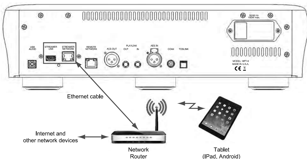
Stream-X2 connections on back panel of MPT-8
